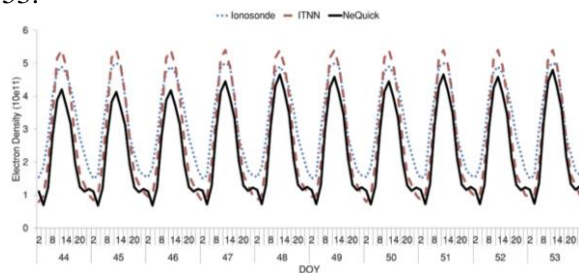
Fig. 7. Comparison of daily variation of electron density ( 10^{11} ele./ m^3 ) at 10 days (44 to 53) for ITNN, ionosondee, and NeQuick models over PRUH ionosondee station at an altitude of 350 km.
