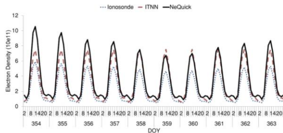
Fig. 6. Comparison of daily variation of electron density ( 10^{11} ele./ m^3 ) at 10 days (354 to 363) for ITNN, ionosondee, and NeQuick models over PRUH ionosondee station at the altitude of 350 km.
