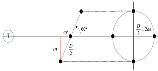
Figure 16: Halo formation [23]
