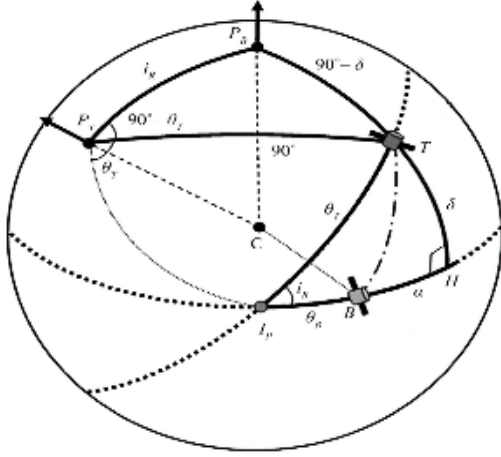
Figure 7: Calculation geometry \alpha and \delta [19]. The angle \delta is obtained from the spherical triangle \Delta P_B P_T I_P . By applying the law of cosines for the sides of the spherical triangle, we reach the following equation.
